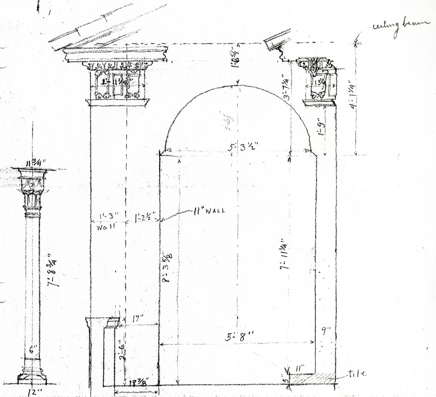
MEASURED DRAWING OF END OF LOGGIA AND OF MOORISH COLUMN BESIDE SPANISH WELL - SCALE \frac{1}{2}" = 1'-0"
