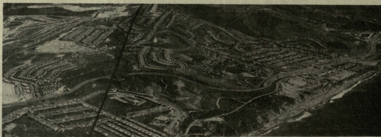
The San Andreas fault (black line) cutting through the Daly City Area south of Mussel Rock.
