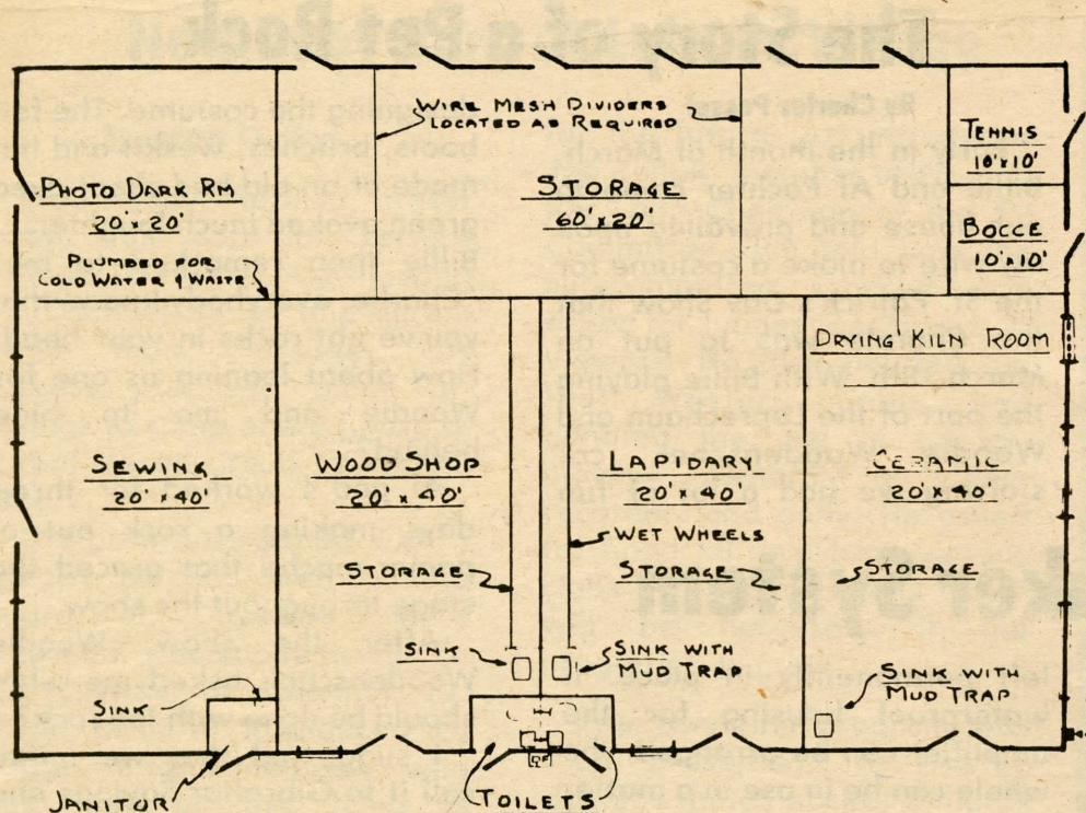
Building Plans
