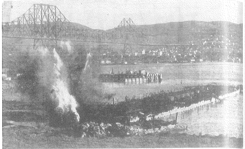
BEGINNING OF THE END for the old train-ferry—nearly 500 feet in length, and one of the longest in the world—started this week for the old bulk resting on the mud of Carquinez Straits offshore from the California Maritime Academy at Morrow Cove. The remains of the old ferry is the subject for a series of dynamite-blasting experiments
