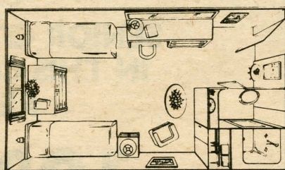
TYPICAL "AA" OR "A" STATEROOM CRUISE VESSEL "SAVANNAH"
