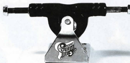
GullWing Cruisers (30°/60°) 9"
