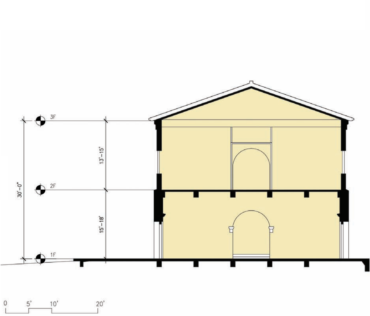
2-Story Building Section
