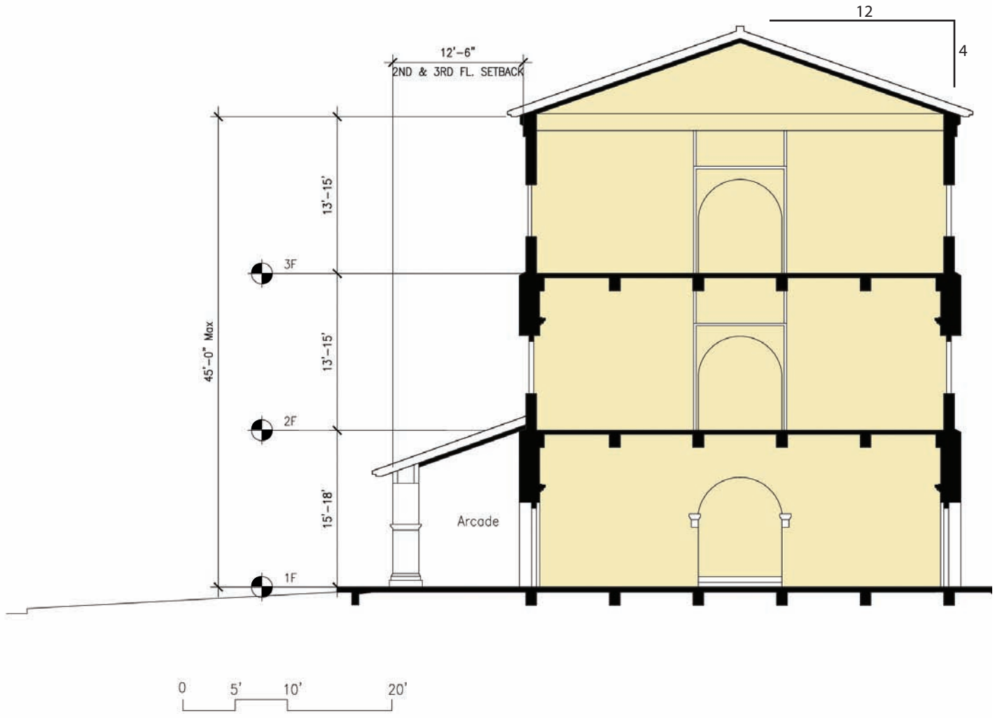
3-Story Building with Arcade
